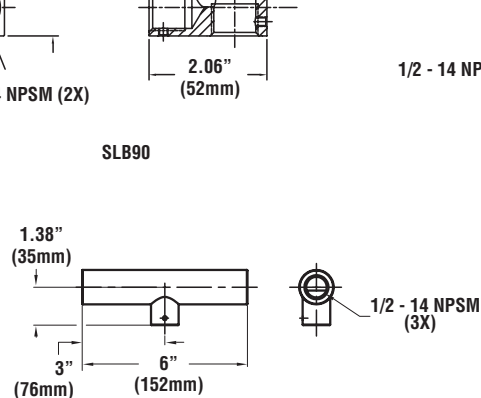
TMA - TWIN MOUNT ADAPTER
